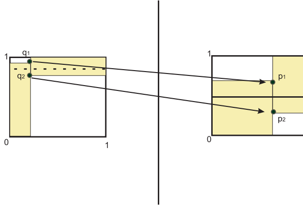
The dynamics on the support
