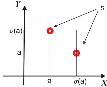
Support of \hat{\mu} in the periodic case.
