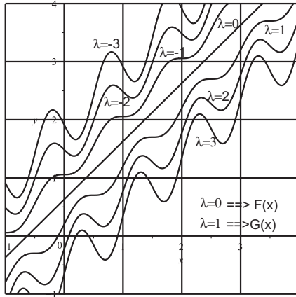
Path of C^r maps F_\lambda ( \lambda -foliation).
