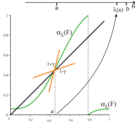
The set Z_\gamma^n(F) .
